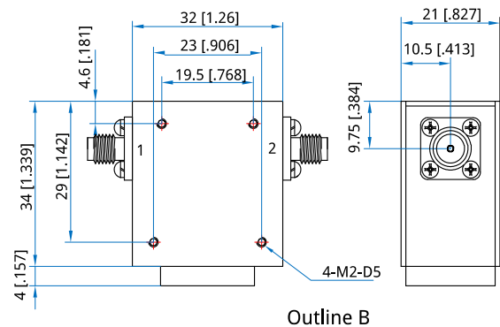
Outline B
